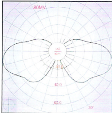
INTENSITY DISTRIBUTION
