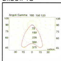
MATT SATIN DOUBLE(+MD) 2x36w T8
