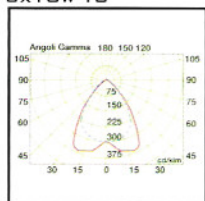
SPECULAR DOUBLE(+SD) 3x18w T8
