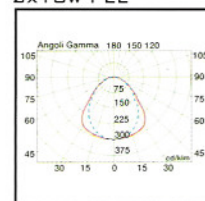
WHITE PREPAINTED SINGLE(+WS) 2x18w PLL
