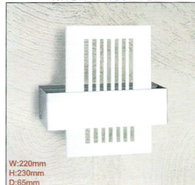
CAT.NO. DI-2001-13/18/26 PLC 1x13w/18w/26w PLC
