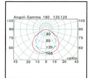
2x55W PLL
