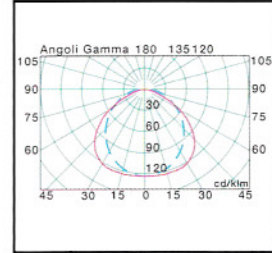
2x55W PLL
