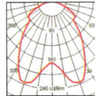
CAT.No. KI-460-213+FG FLOATING GLASS 2x13w PLC 沿浮玻璃
