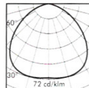
MII-6012 1x20W 12V
