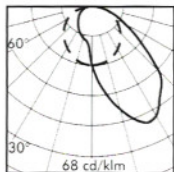
MII-6007 1x10W PLC
