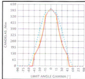
1000W HALOGEN
