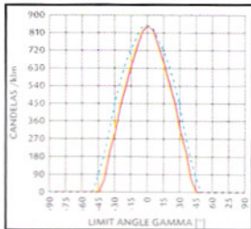
500W HALOGEN
