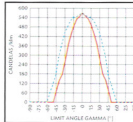
1500W HALOGEN
