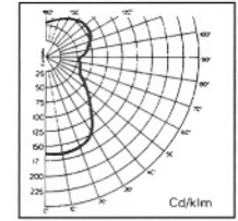
DOUBLE LAMP W/ PRISMATIC 孖管 + 膠罩
