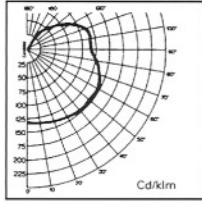
SINGLE LAMP 單管
