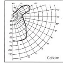
SINGLE LAMP W/ PRISMATIC 單管 + 膠罩
