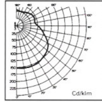
DOUBLE LAMP 孖管
