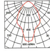
CAT.No. RI-1018-126+FG+C VERTICAL W/ FLAT CLEAR GLASS 1x26w PLC
