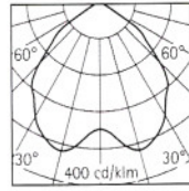
CAT.No. RI-9490-226 HORIZONTAL OPEN 2x26w PLC
