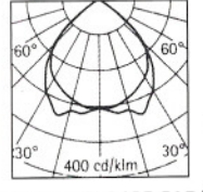
CAT.No. RI-9490-218+CL HORIZONTAL W/ CROSS LOUVER 2x18w PLC
