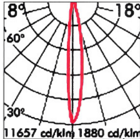
DOWN LIGHT 向下照射 1x70w HIT
