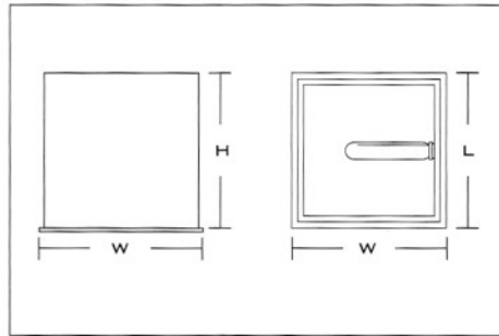
DIMENSION - RECESSED-MOUNTED 尺寸 - 暗裝
