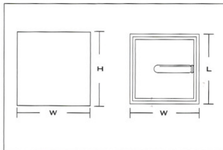
DIMENSION - SURFACE-MOUNTED 尺寸 - 明裝
