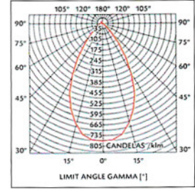
PRISMATIC 250w HSE
