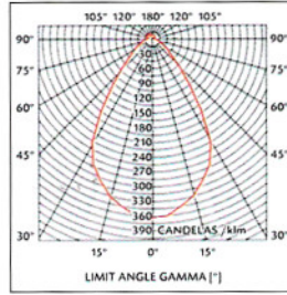
PRISMATIC 150w HIE
